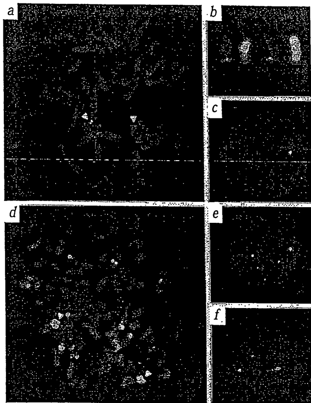
Fig. 2 Dual colour FISH demonstrating localization of the STK15 probe (green signals) along with chromosome-20-specific centromeric probe or a 'p' arm-specific probe (red signals) on normal human chromosome 20 (a, b) and diploid copy number of STK15 in the interphase nucleus of normal breast epithelial tissue (c). Amplification of STK15 was detected by single colour FISH using FITC-labelled STK15 probe (yellow signals) on chromosomes of human breast cancer cell line BT474 (d) and dual colour FISH using FITC-labelled STK15 probe (green signals) along with Cy3-labelled chromosome 20 'p' arm probe (red signals) in interphase nuclei of primary human breast tumour tissues (e, f). Note multiple STK15 signals in contrast with two signals for the 'p' arm probe in the nuclei.
